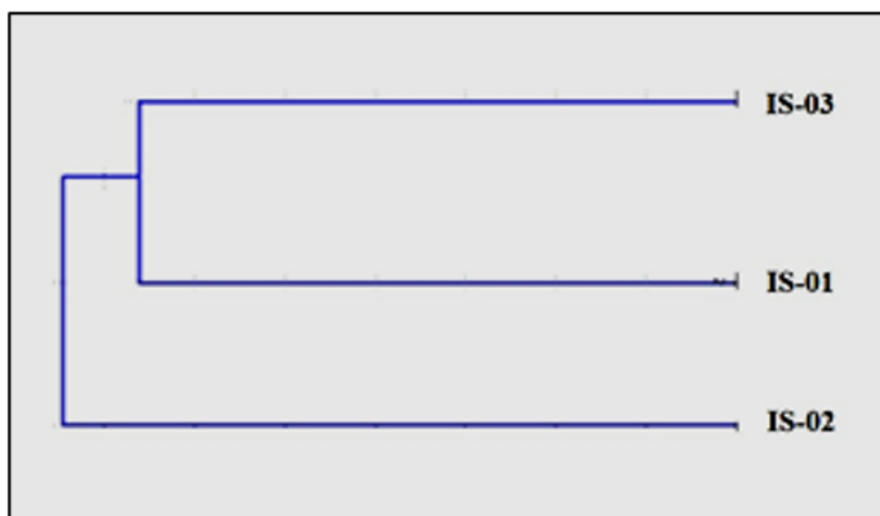
Fig. 16: Dendrogram shows the genetic relationship between the three bacterial isolates based on analysis of DNA polymorphisms produced via ISSR method using eight primers.
