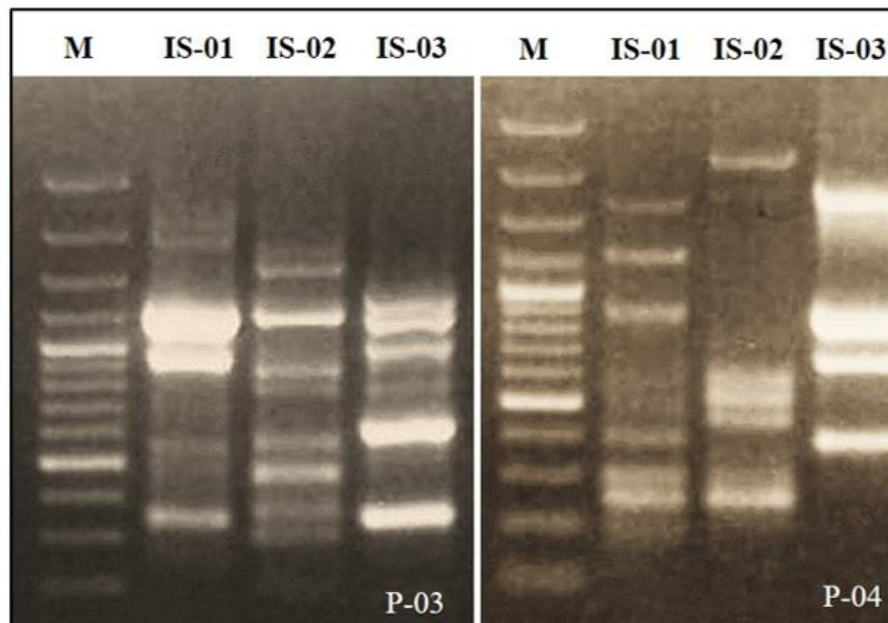
Fig.13: Agarose gels (1.2%) stained with ethidium bromide show DNA polymorphisms of three bacterial isolates amplified using P-03 and P-04 primers among ISSR method.
